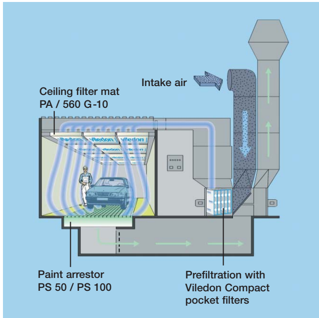
Fig. 3 Schematic depiction of a repair cabin
