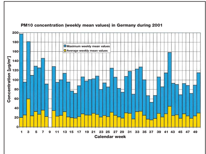
Fig. 1 Airborne particle concentration in Germany during 2001
