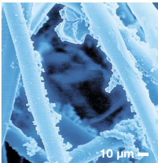
Fig. 6 Fibers with an actively adhesive finish, showing the retained particles
