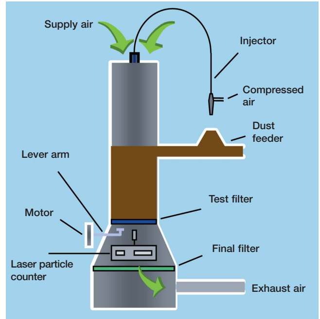
Fig. 7 Filter test rig for the migration test
