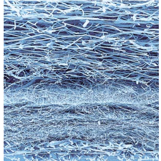
3-layer nonwoven filter medium, 500 \mu\text{m} inner layer electrostatically spun microfibers (TFP95)
