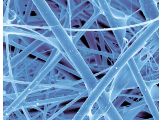
High-strength glassfiber filter medium 20 µm with a special thermoplastic bonding system
