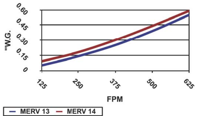
15" Deep Resistance to Airflow
