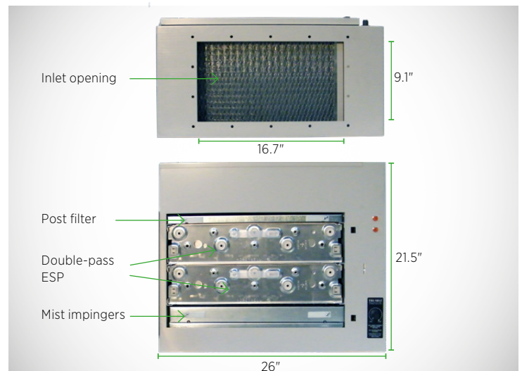
Top: View from below Tri-Mist 850 G2. Bottom: Internal view
